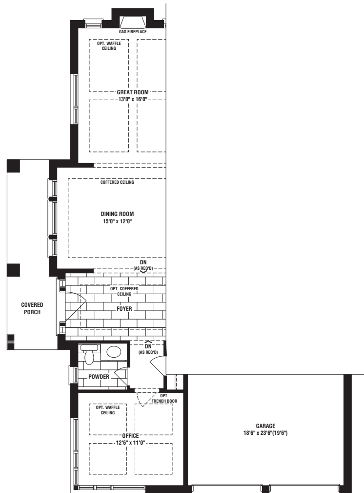
PARTIAL GROUND FLOOR ELEV. 'C'
