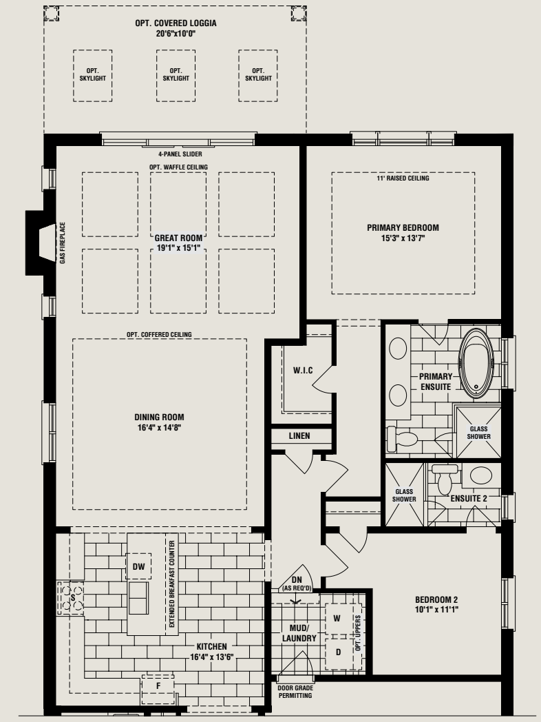
PARTIAL OPT. GROUND FLOOR PLAN ELEV. 'A' (ELEV. 'B' & 'C' SIMILAR)
