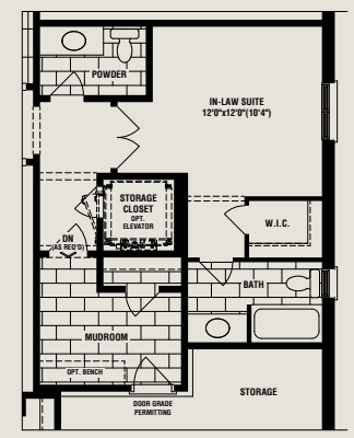
PARTIAL OPT. IN-LAW SUITE ELEV. 'A' (ELEV. 'B' & 'C' SIMILAR)
