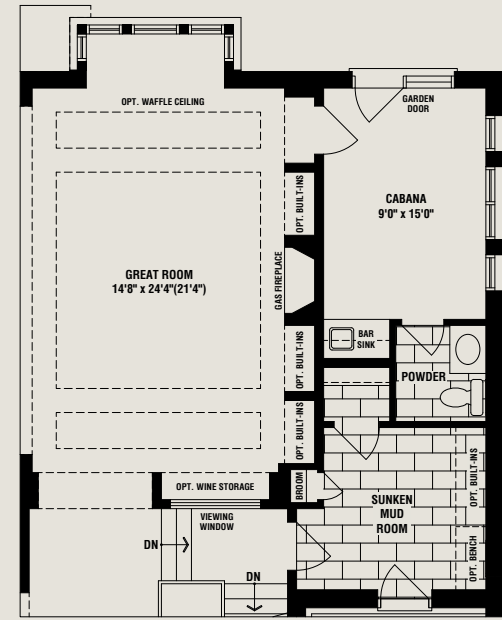
PARTIAL OPT. GROUND FLOOR PLAN W/ CABANA
